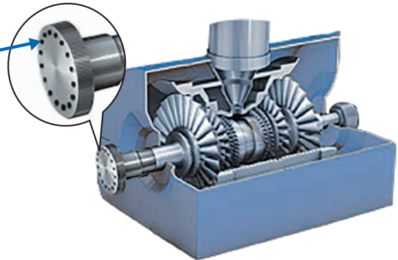
Turbine rotor
