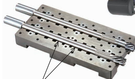
PF Radical Mill Reamer with Guide and Oil Hole
