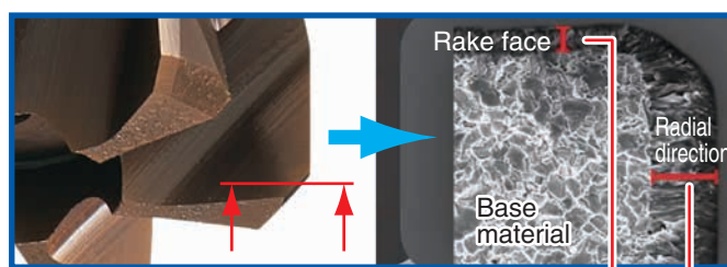
Non-uniform coating film thickness
