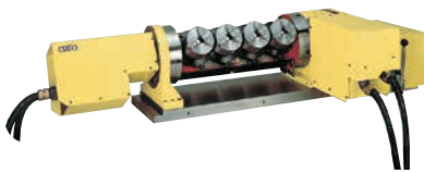
4" Power chuck in photo is optional.
