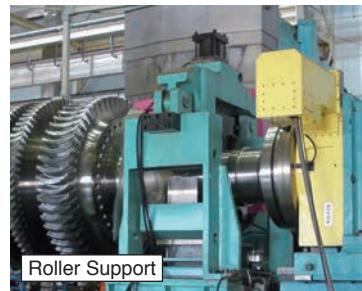
CNC1201 Indexing of the turbine shaft. Turbine shaft is supported and clamped by the roller support.
