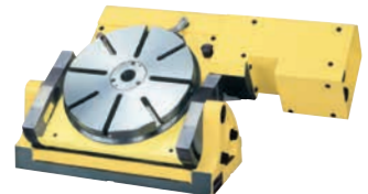
NST manual tilting rotary table
