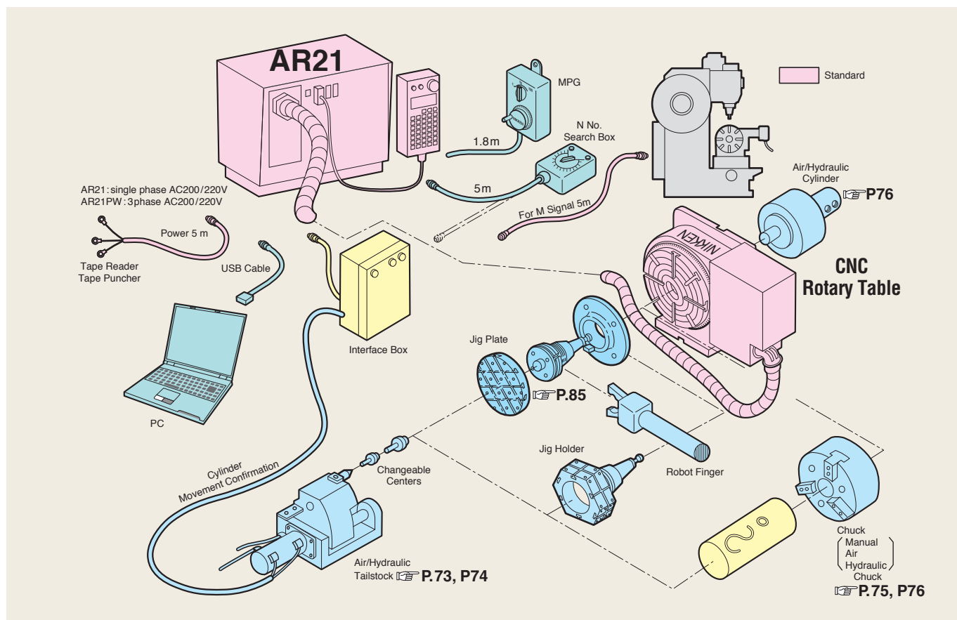
AR21 controller for larger capacity • 4.4KW is available. • 3 phase AC200/220V
