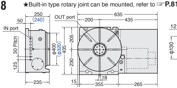
Rotary joint shown in photo is optional.
