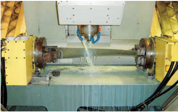
Synchronous Rotation by CNC401 X 2units
