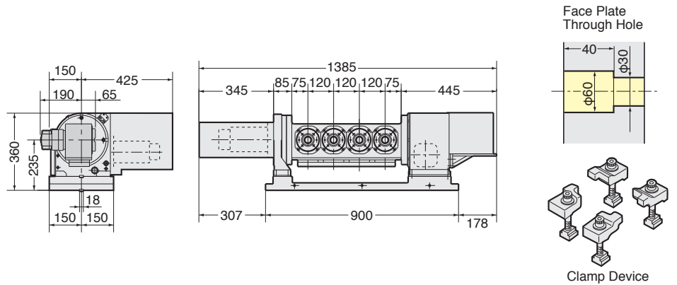
4" Power chuck in photo is optional.
