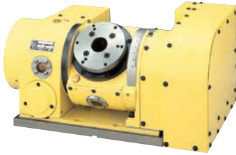
Photo with \phi 130 mm plate. (Standard accessories)
