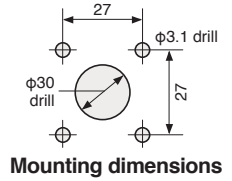
Mounting dimensions
