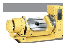
5AX P56 5AX-T400, B450
